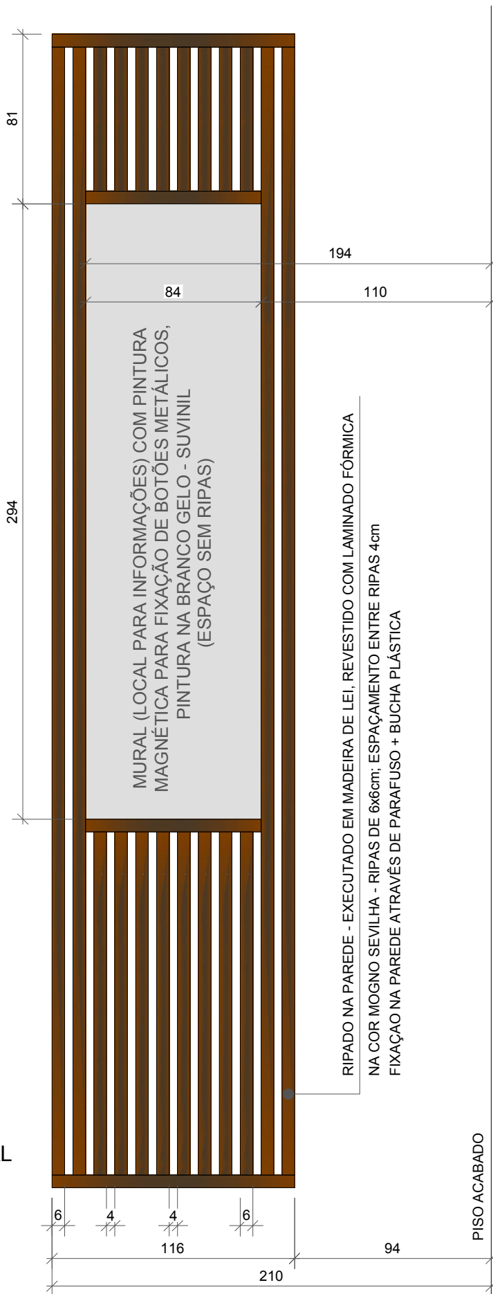
VISTA FRONTAL
